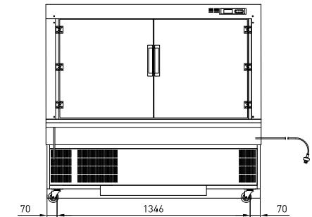
REAR VIEW
