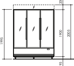
Integral front elevation
