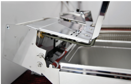
Unique tilt-back fryer heads can be removed or locked
